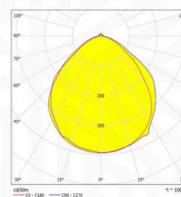
Luminance Distribution
